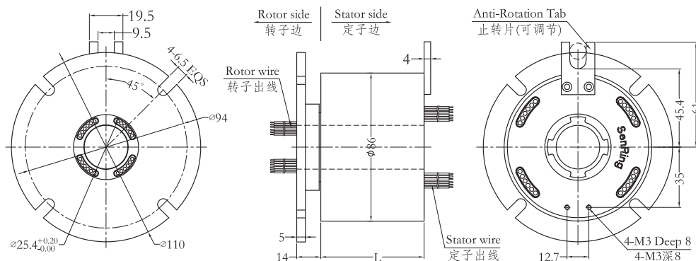
H2586F series model list Part no. Circuits Length L(mm) Part no. Circuits Length L(mm) 10A Signal or 0~5A 10A Signal or 0~5A H2586F-02S 0 2 32 H2586F-1210-12S 12 12 120 H2586F-0210 2 0 32 H2586F-1810-06S 18 6 120 H2586F-03S 0 3 36 H2586F-2410 24 0 120 H2586F-0310 3 0 36 H2586F-30S 0 30 144 H2586F-06S 0 6 48 H2586F-0610-24S 6 24 144 H2586F-0210-04S 2 4 48 H2586F-1210-18S 12 18 144 H2586F-0410-02S 4 2 48 H2586F-1810-12S 18 12 144 H2586F-0610 6 0 48 H2586F-2410-06S 24 6 144 H2586F-12S 0 12 72 H2586F-3010 30 0 144 H2586F-0210-10S 2 10 72 H2586F-36S 0 36 168 H2586F-0310-09S 3 9 72 H2586F-0610-30S 6 30 168 H2586F-0610-06S 6 6 72 H2586F-1210-24S 12 24 168 H2586F-0810-04S 8 4 72 H2586F-3610 36 0 168 H2586F-1010-02S 10 2 72 H2586F-42S 0 42 192 H2586F-1210 12 0 72 H2586F-0610-36S 6 36 192 H2586F-18S 0 18 96 H2586F-1210-30S 12 30 192 H2586F-0210-16S 2 16 96 H2586F-48S 0 48 216 H2586F-0410-14S 4 14 96 H2586F-0610-42S 6 42 216 H2586F-0610-12S 6 12 96 H2586F-1010-38S 10 38 216 H2586F-0810-10S 8 10 96 H2586F-1210-36S 12 36 216 H2586F-1010-08S 10 8 96 H2586F-1810-30S 18 30 216 H2586F-1210-06S 12 6 96 H2586F-2410-24S 24 24 216 H2586F-1410-04S 14 4 96 H2586F-60S 0 60 264 H2586F-1610-02S 16 2 96 H2586F-0610-54S 6 54 264 H2586F-24S 0 24 120 H2586F-1010-50S 10 50 264 H2586F-0410-20S 4 20 120 H2586F-1210-48S 12 48 264 H2586F-0610-18S 6 18 120 H2586F-72S 0 72 312
